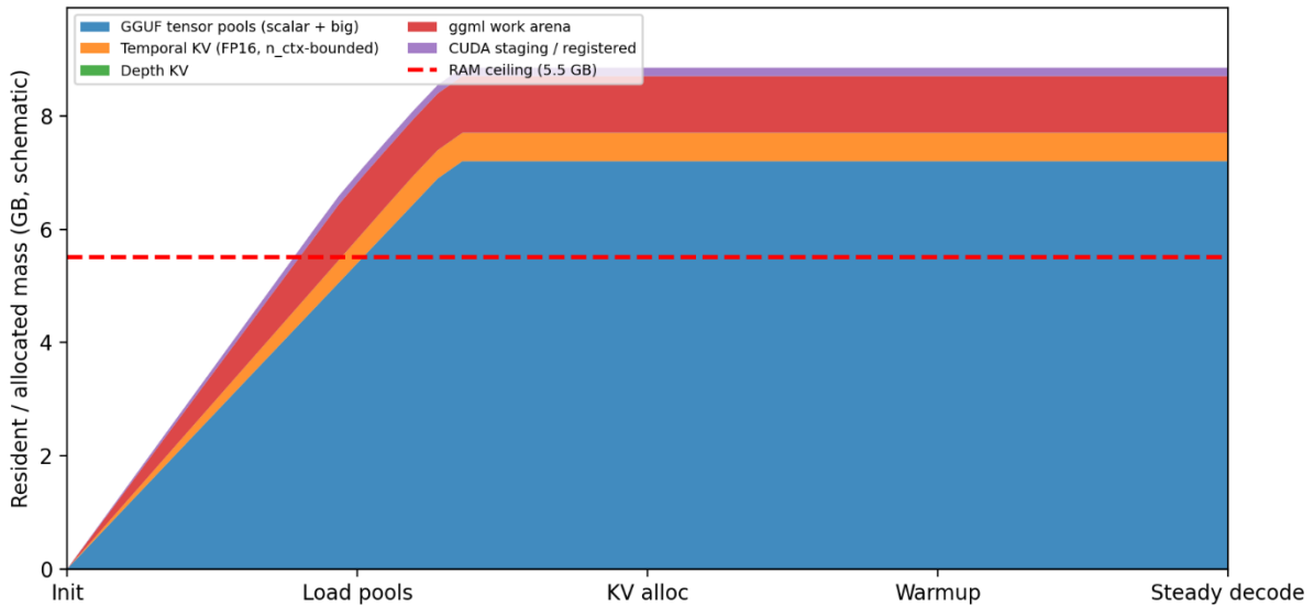
Figure 7 Resident set size vs. usable RAM on Jetson Orin Nano 8 GB (25 W). Schematic RSS time series under the current pread + cudaHostRegister loader (not lazy weight mmap): (i) fully resident GGUF pools, (ii) FP16 temporal KV ( n_{\text{ctx}} \leq 1024 ), (iii) depth KV, (iv) fixed 1 GiB ggml work arena, (v) CUDA staging / registered buffers. Total residency exceeds the ~5.5 GB nominal usable ceiling, so the device additionally relies on a configured 8 GiB swapfile plus zram-backed compressed swap to absorb the overshoot — explaining why the model loads and runs at the cost of paging-induced ~800 ms decode latency rather than OOM-killing.
