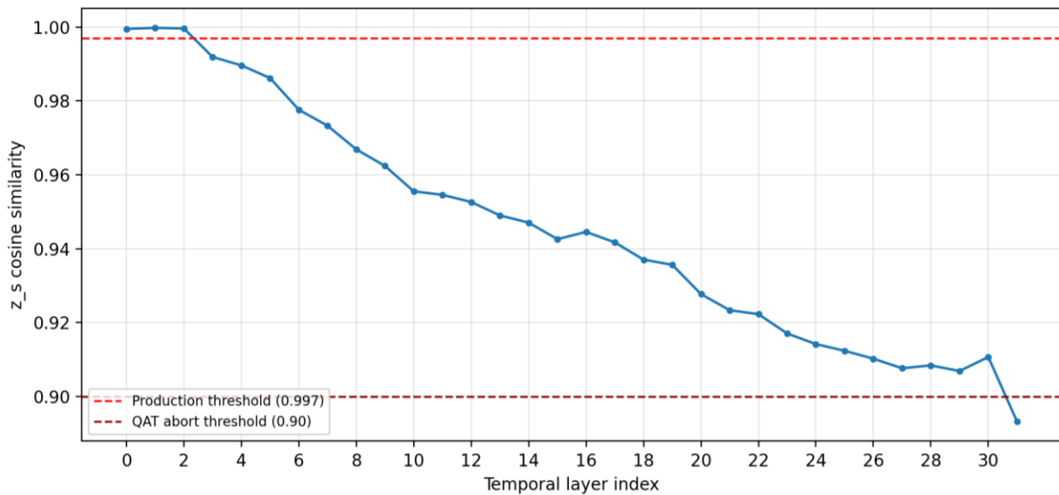
Figure 6 v11 Cosine Cascade
