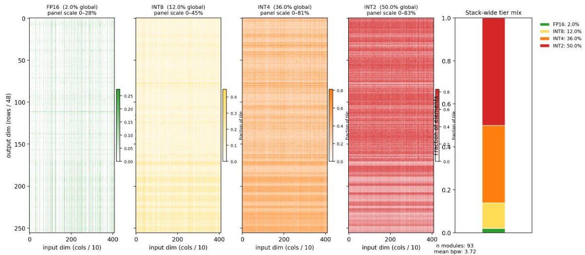
Figure 4 SEPTQ within-tensor tier assignment for a representative module ( L0.self_attn.in_proj_weight ). Each of the four panels shows the local fraction-per-tile of one precision tier within the downsampled weight matrix ( 256 \times 384 tiles, \sim 48 \times 11 weights per tile). Bright regions in the FP16 (green) panel correspond to output dimensions where the Hessian-saliency router concentrated full-precision weights — these align with the activation-outlier channels discussed in §Performance Analysis. The progression \text{FP16} \rightarrow \text{INT8} \rightarrow \text{INT4} \rightarrow \text{INT2} traces the gradient from “few, high-precision” outlier rows to “bulk, aggressively quantized” non-salient weights. The side panel reports the stack-wide tier mix (2 / 12 / 36 / 50 %) yielding a mean 3.72 effective bits-per-weight across all 93 quantized modules.
